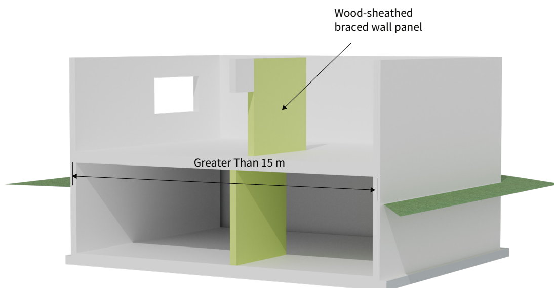
Figure 3.8: Braced Wall Panels in the Basement
