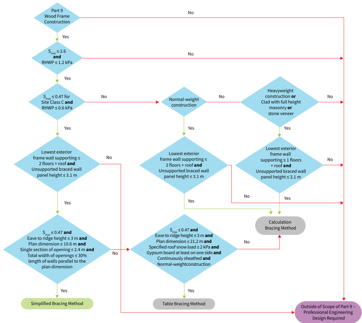
Figure 3.1: Flowchart for the Determination of Seismic Bracing Requirements for Part 9 Wood-frame Construction
