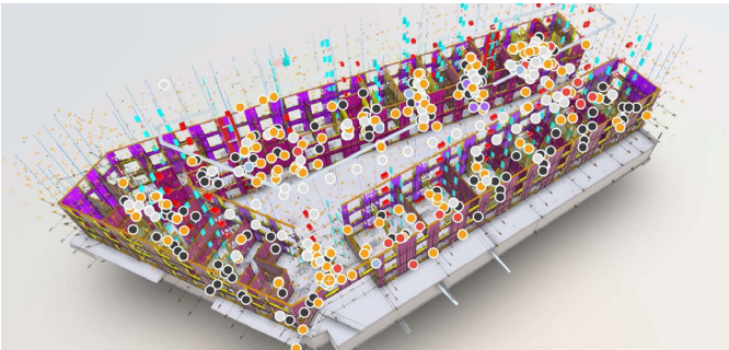
Figure 9. BIM model clash detection during model coordination (source: Public Architecture)
